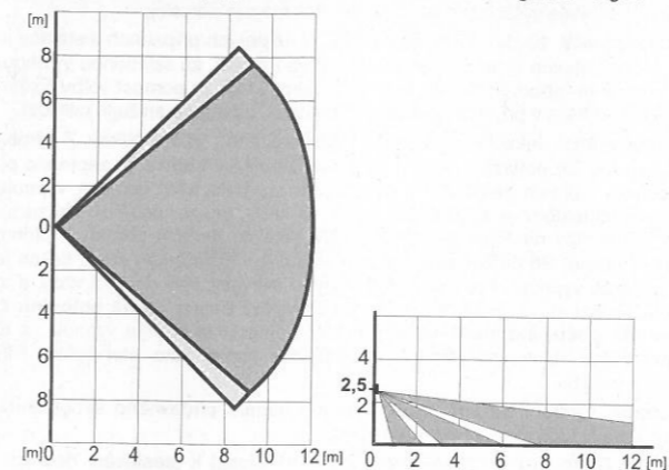
Fig 2: detection characteristic.
