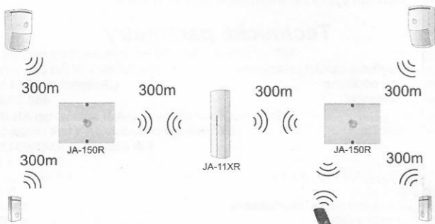
Figure 1: Extension of communication range
