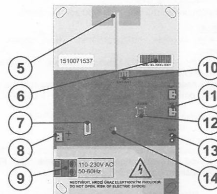
Figure 3: 5 - antenna; 6 - production code; 7 - mini USB connector; 8 - backup battery connector; 9 - mains terminals and protective foil; 10 - external antenna connector; 11 - tamper contact connectors; 12 - LEARN button; 13 - MAN terminal for manual boot from powered backup battery; 14 - LED indicators
